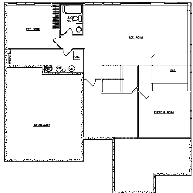
Lower Level Floor Plan
